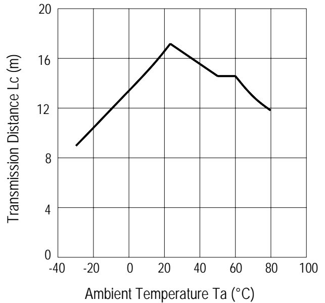
Fig.-9 Arrival Distance vs. Ambient Temperature
