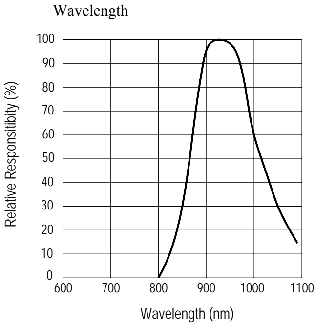
Fig.-4 Relative Spectral Sensitivity vs.
