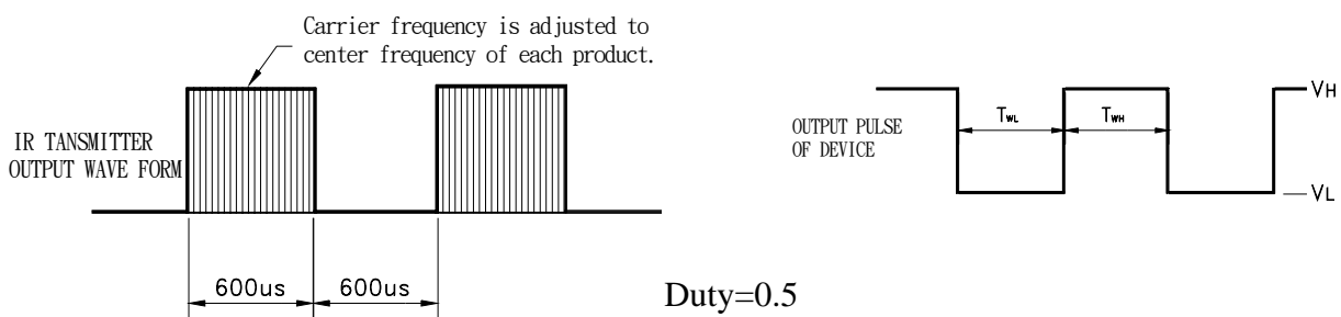
Fig.-1 Transmitter Wave Form
