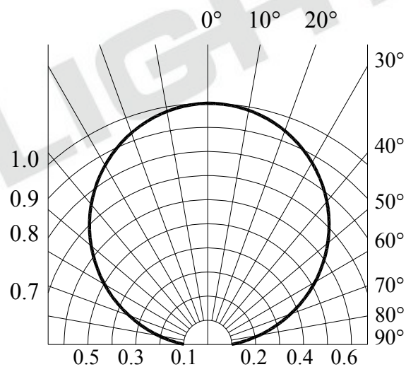
Fig.6 - Radiation Diagram
