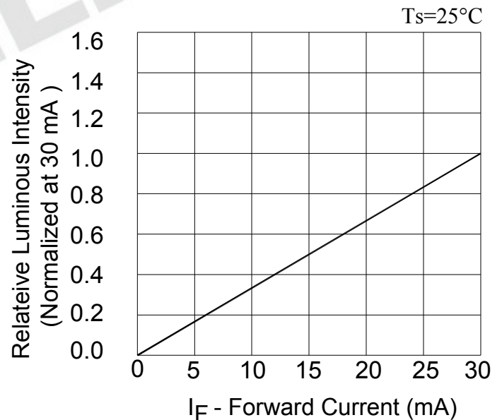
Fig.2 - Relative Luminous Intensity vs. Forward Current
