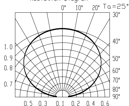
Radiation Diagram
