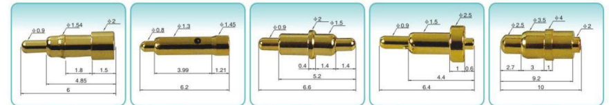
JCPG271 2X6 JCPG272 1.45X6.2 JCPG273 2X6.6 JCPG274 2.5X6.4 JCPG275 4X10
