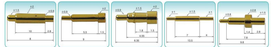
JCPG296 1.45X8 JCPG297 2X9 JCPG298 2X6.35 JCPG299 1.5X13.5 JCPG300 2.8X9.8
