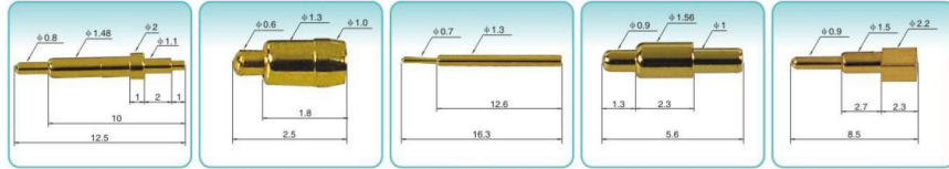
JCPG261 2X12.5 JCPG262 1.3X2.5 JCPG263 1.3X16.3 JCPG264 1.56X5.6 JCPG265 2.2X1.5X8.5
