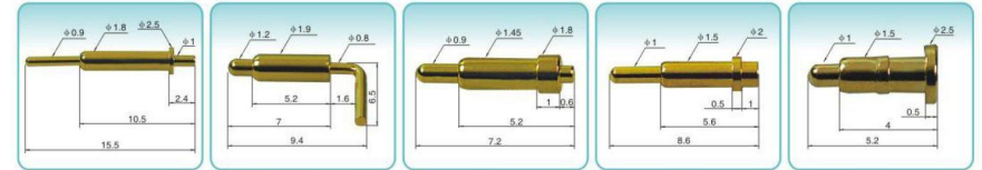
JCPG286 2.5X15.5 JCPG287 1.9X9.4 JCPG288 1.8X7.2 JCPG289 2X8.6 JCPG290 2.5X5.2
