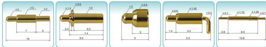
JCPG266 3X16 JCPG267 3.5X9.5 JCPG268 3.5X5 JCPG269 1.45X5.4 JCPG270 1.25X13.6
