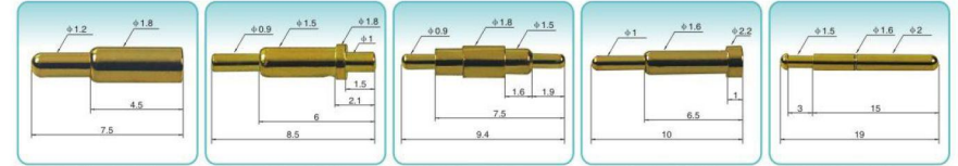
JCPG291 1.8X7.5 JCPG292 1.8X8.5 JCPG293 1.8X9.4 JCPG294 2.2X10 JCPG295 2X19
