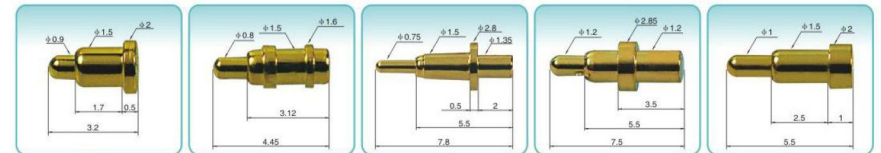
JCPG281 2X3.2 JCPG282 1.6X4.45 JCPG283 2.8X7.8 JCPG284 2.85X7.5 JCPG285 2X5.5
