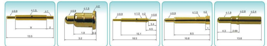
JCPG276 1.5X13.5 JCPG277 2X3.2 JCPG278 2X18.5 JCPG279 2X10.8 JCPG280 8X13.8
