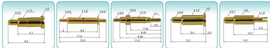
JCPG241 2X5.6 JCPG242 2.5X13.2 JCPG243 2.4X11.5 JCPG244 2X5.3 JCPG245 3X14.1
