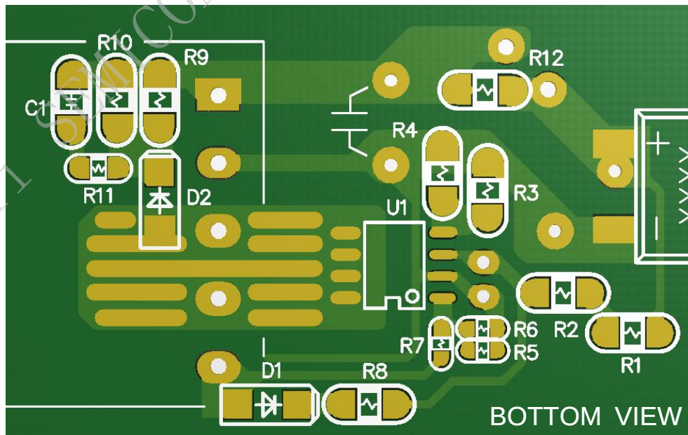
Fig7. Typical layout reference
