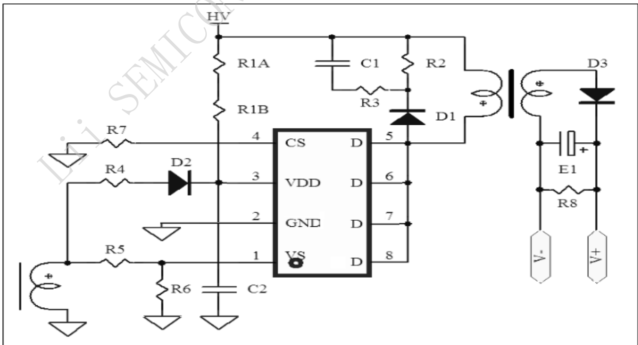
Fig3. Typical Simplified Schematic
