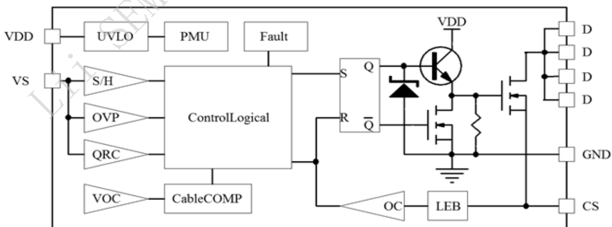
Fig1. Internal functional block diagram
