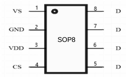
Fig2. Pin Definitions
