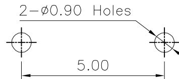
PCB Layout (Pattern Side)
