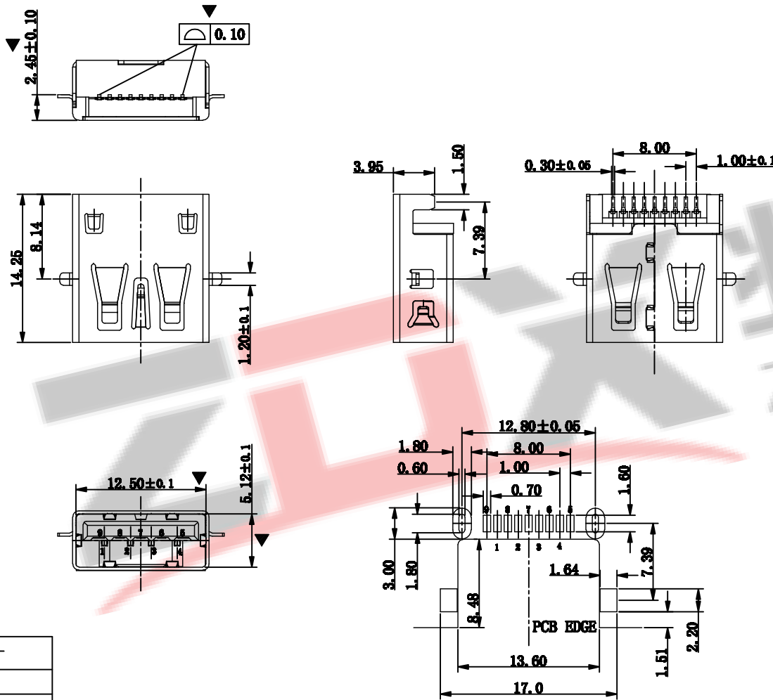
RECOMMENDED PCBA LAYOUT (TOLERANCE: ± 0.05)
