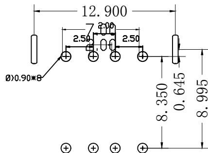
RBCOMMENDBD P. C. B PATTBRN LAY OUT
