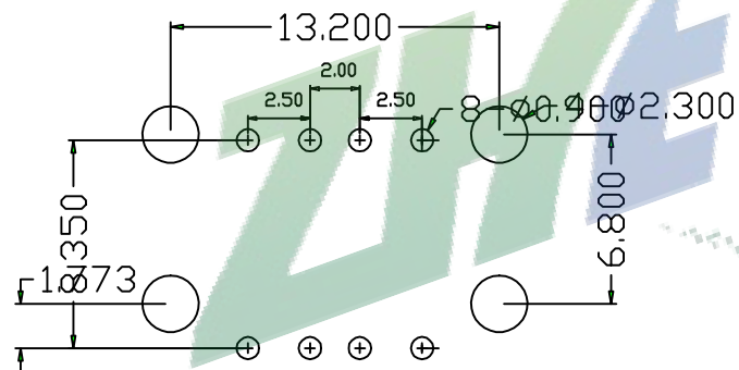
RBCOMMENDBD P.C.B PATTBRN LAY OUT
