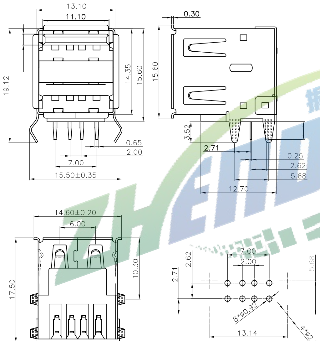
PCB.LAYOUT
